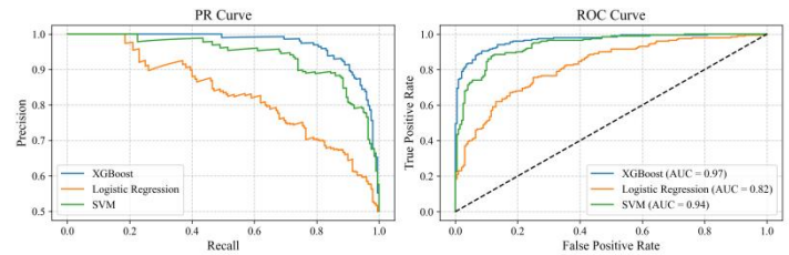
Fig 3. Comparison of PR curves and ROC curves of different models
